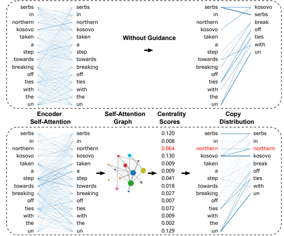
Figure 3: The guidance process for SAGCopy Indegree model, showing that the keyword “northern” is correctly copied for our model.
